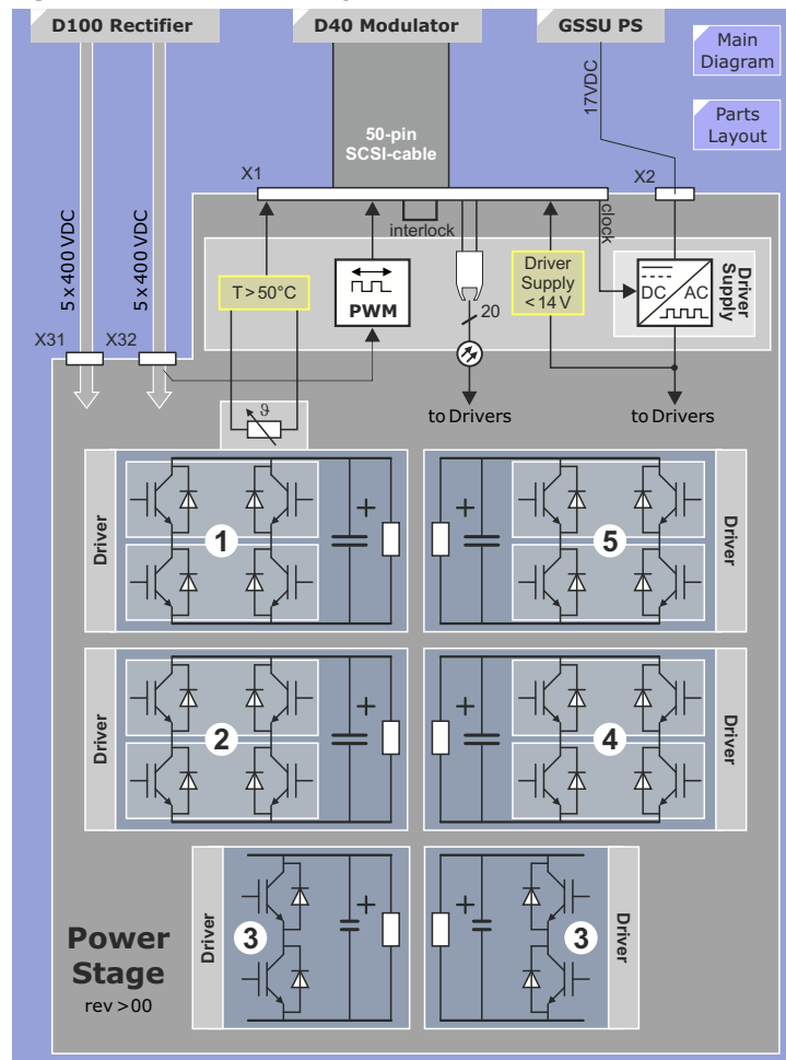
Figure 151 One Power Stage Module
