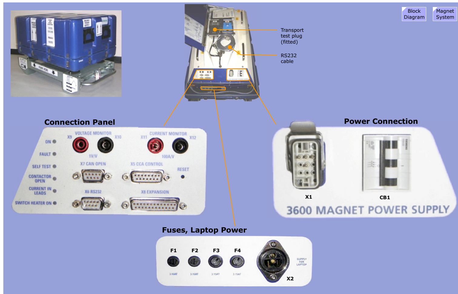
Figure 258 Magnet Power Supply Connections
