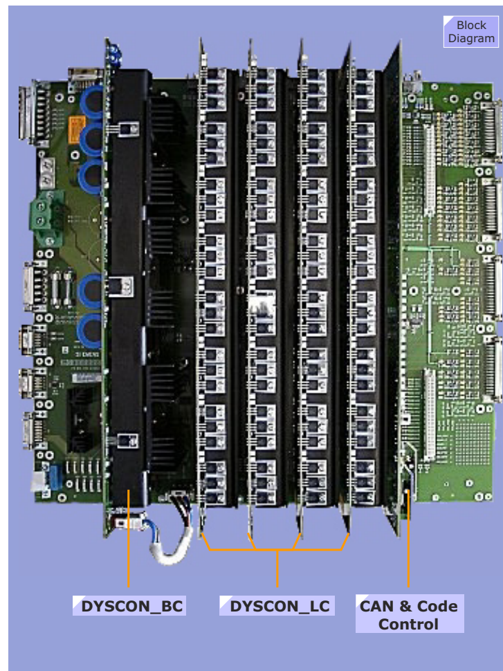
Figure 68 RFIS Assembly
