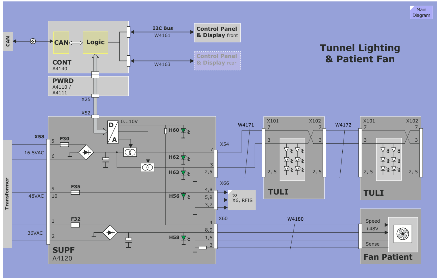
Figure 109 Patient Fan, Tunnel Light and Auxiliary Supply
