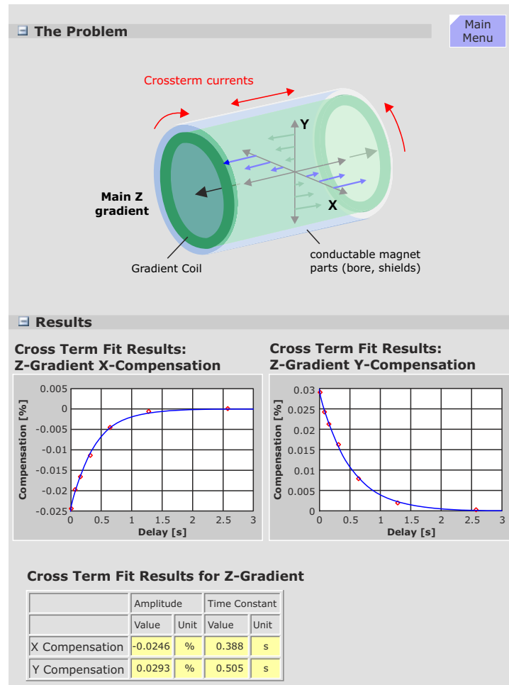
Figure 224 Cross Term Currents
