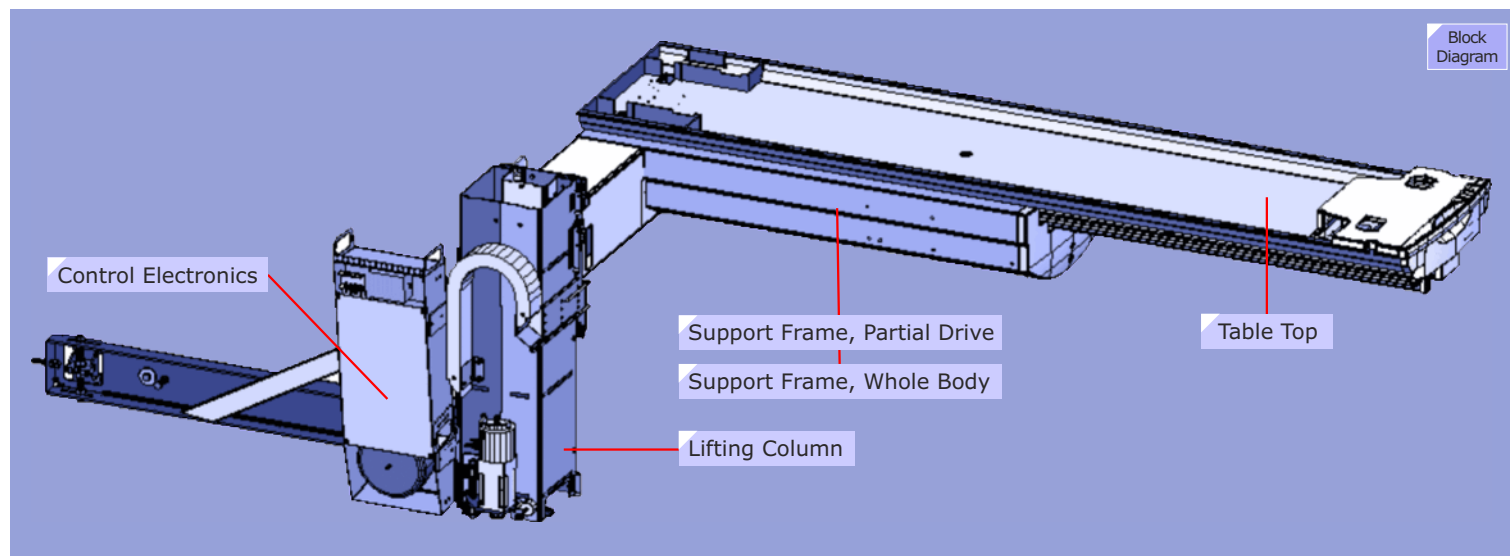
Figure 90 Patient Table Assemblies: Mechanical View
