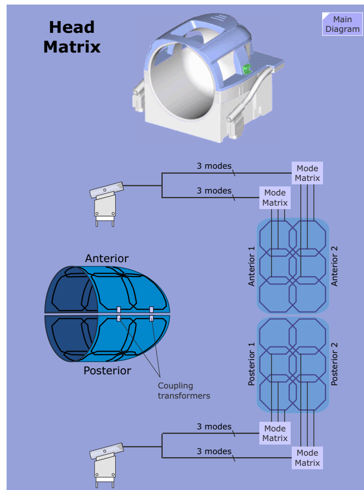
Figure 81 Head Matrix Coil Construction
