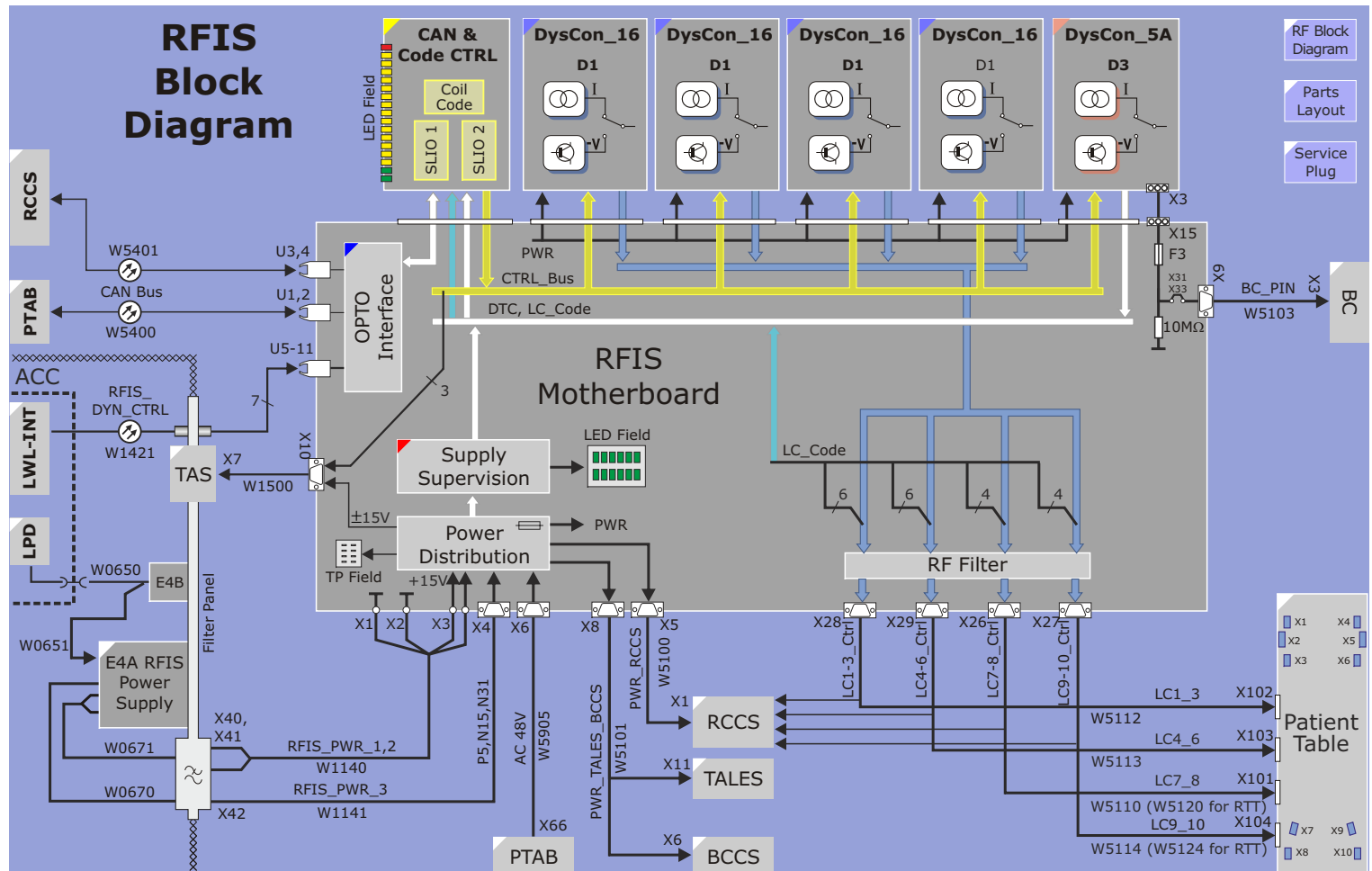
Figure 69 RFIS Block Diagram
