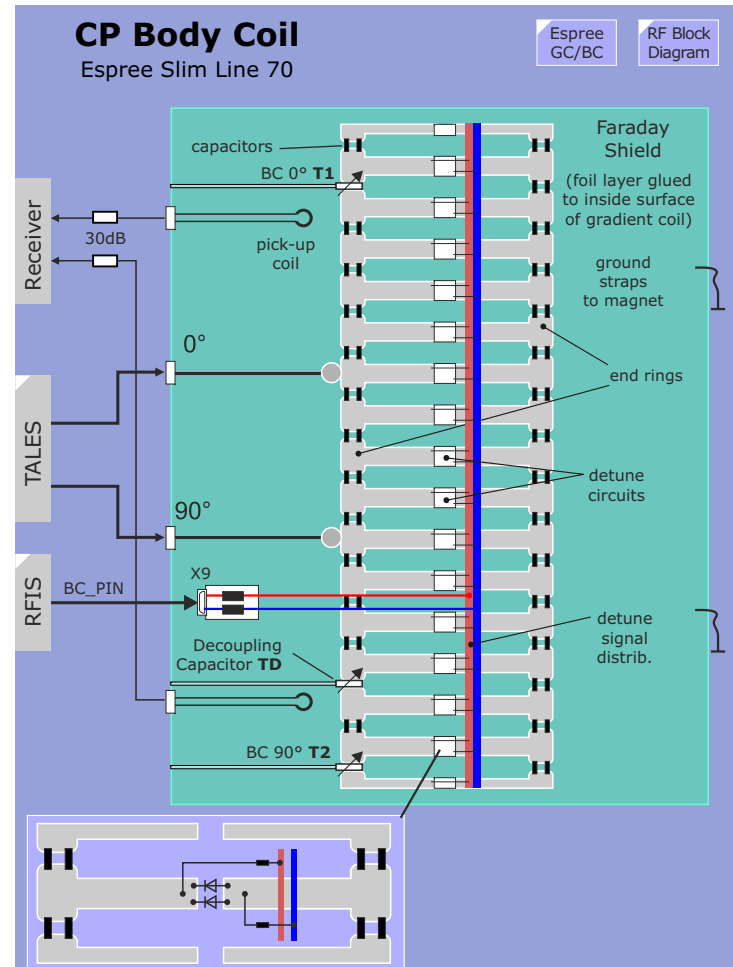
Figure 66 Body Coil Block Diagram
