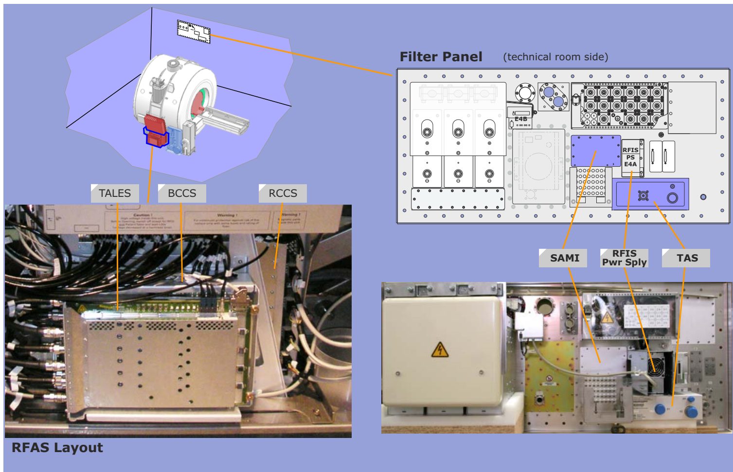
Figure 57 RFAS Parts Layout
