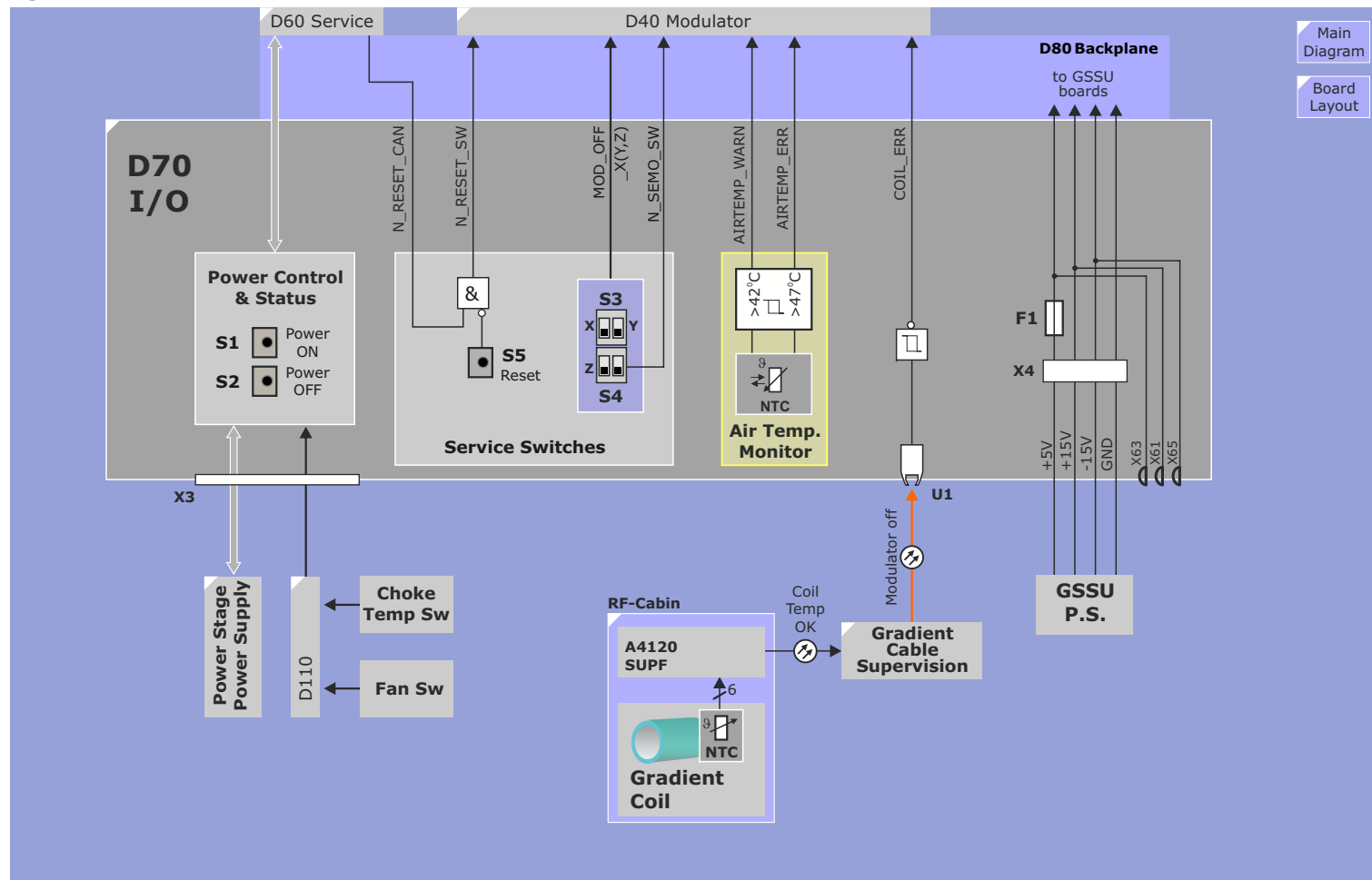
Figure 145 D70 I/O Overview
