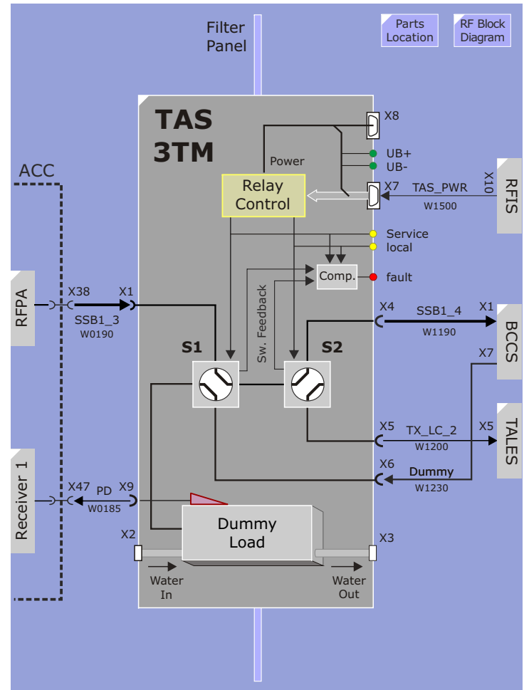
Figure 58 TAS_3TM Block Diagram
