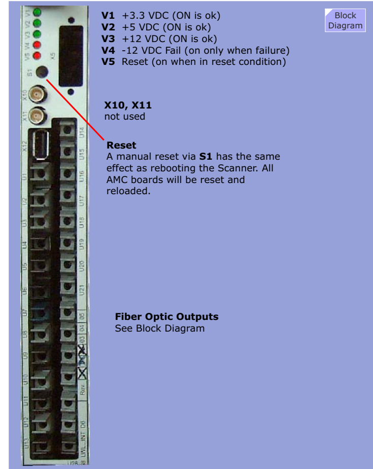
Figure 40 LWL_INT Front View
