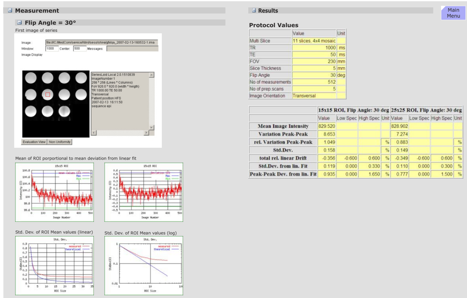
Figure 244 Long Term Stability Check
