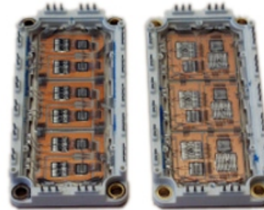
Figure 152 Two switches containing 6 IGBTs each
