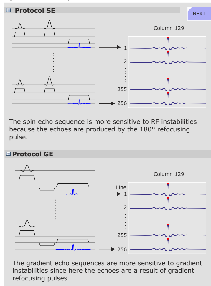
Figure 240 Stability Check Measurement
