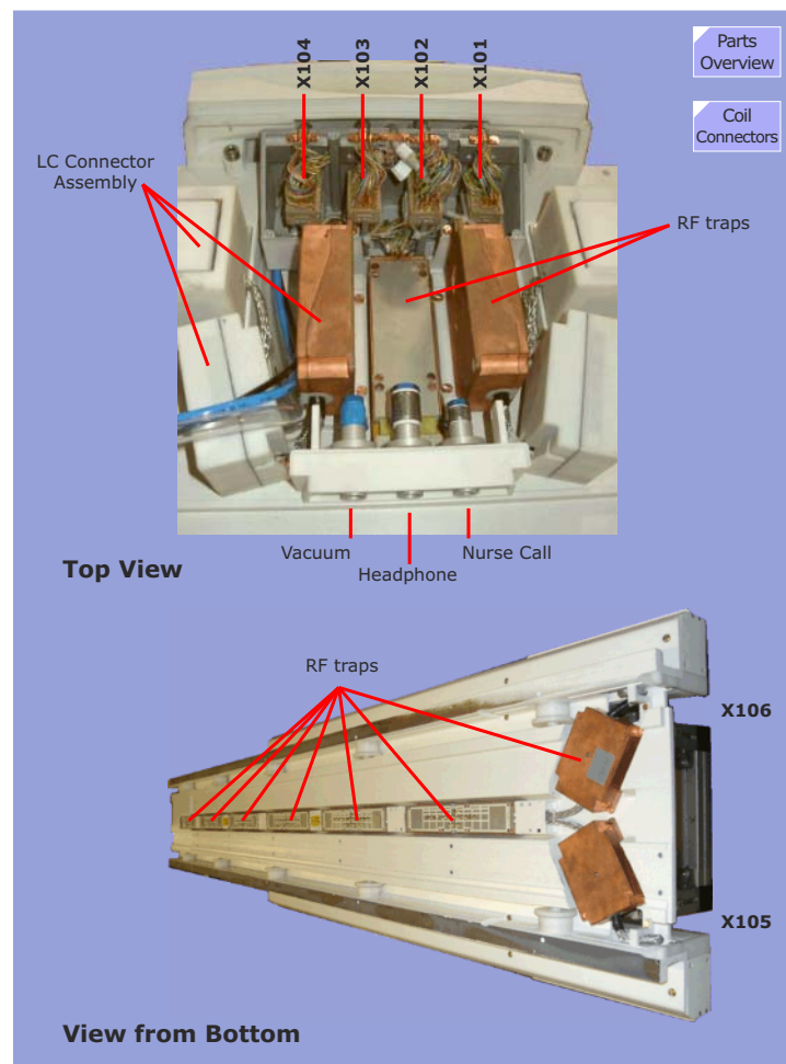
Figure 96 Table Top Assembly
