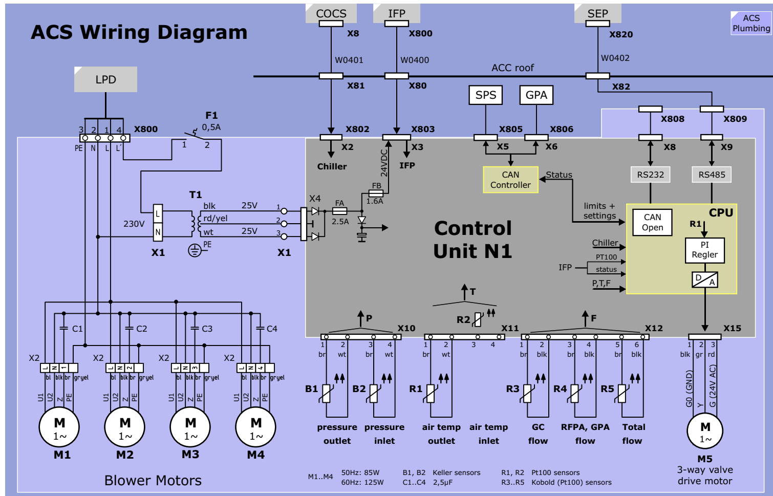
Figure 193 ACS Wiring Diagram
