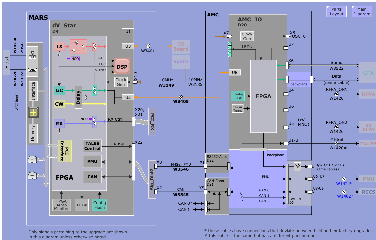
Figure 251 Hardware Overview
