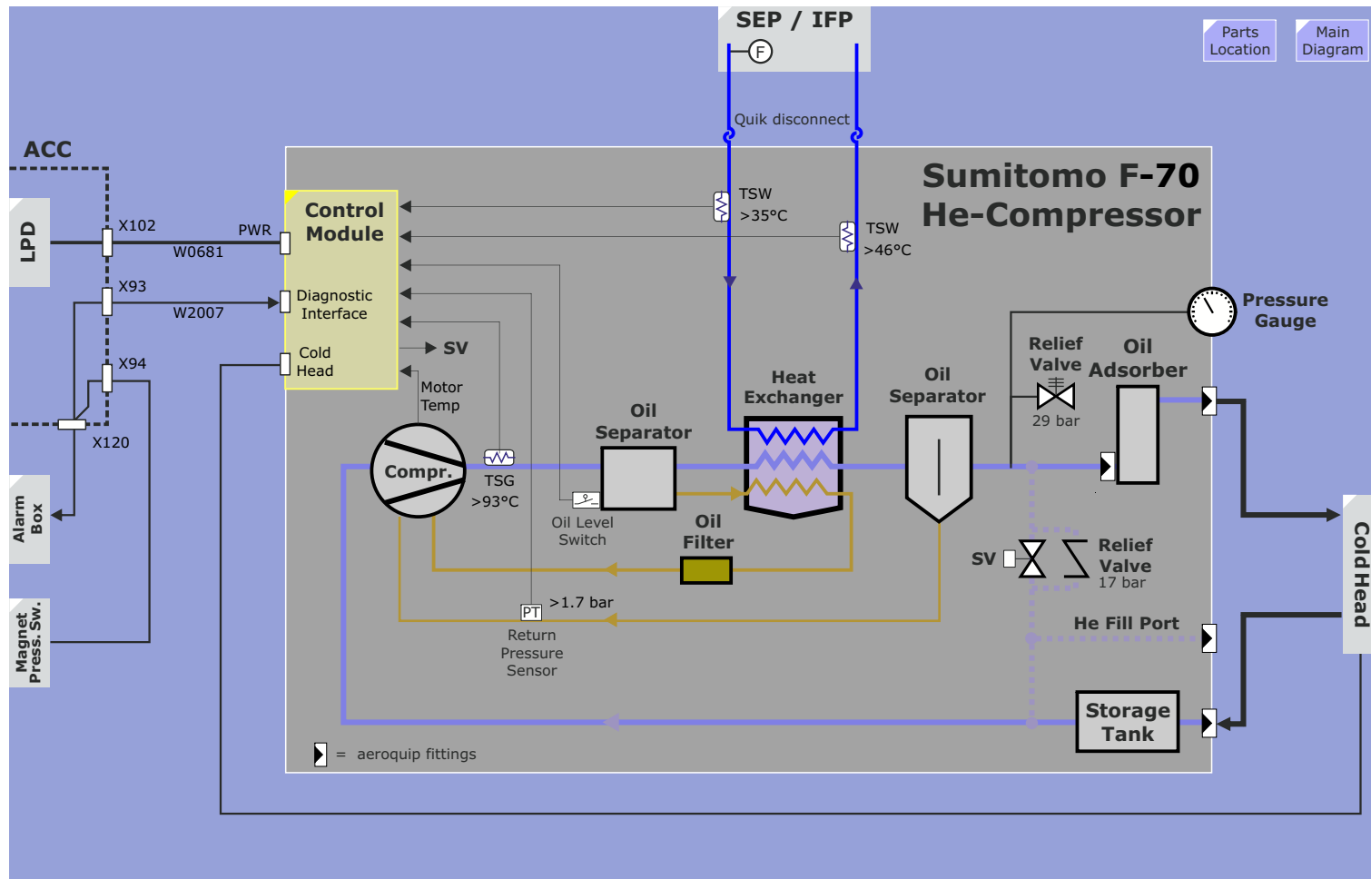
Figure 183 F-70 Compressor Block Diagram
