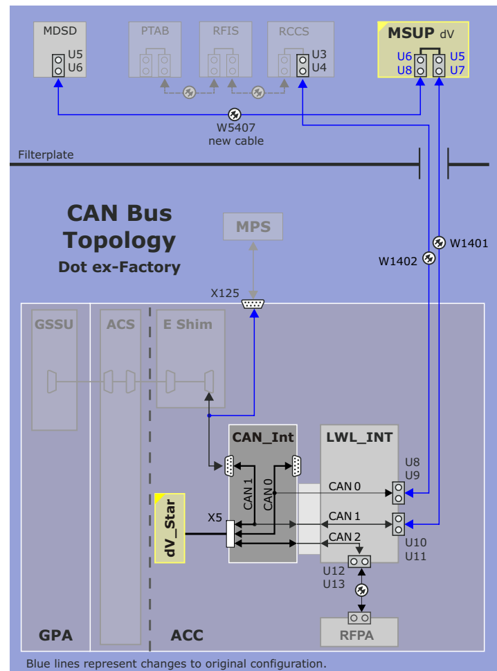
Figure 253 CAN Topology Dot ex-Factory
