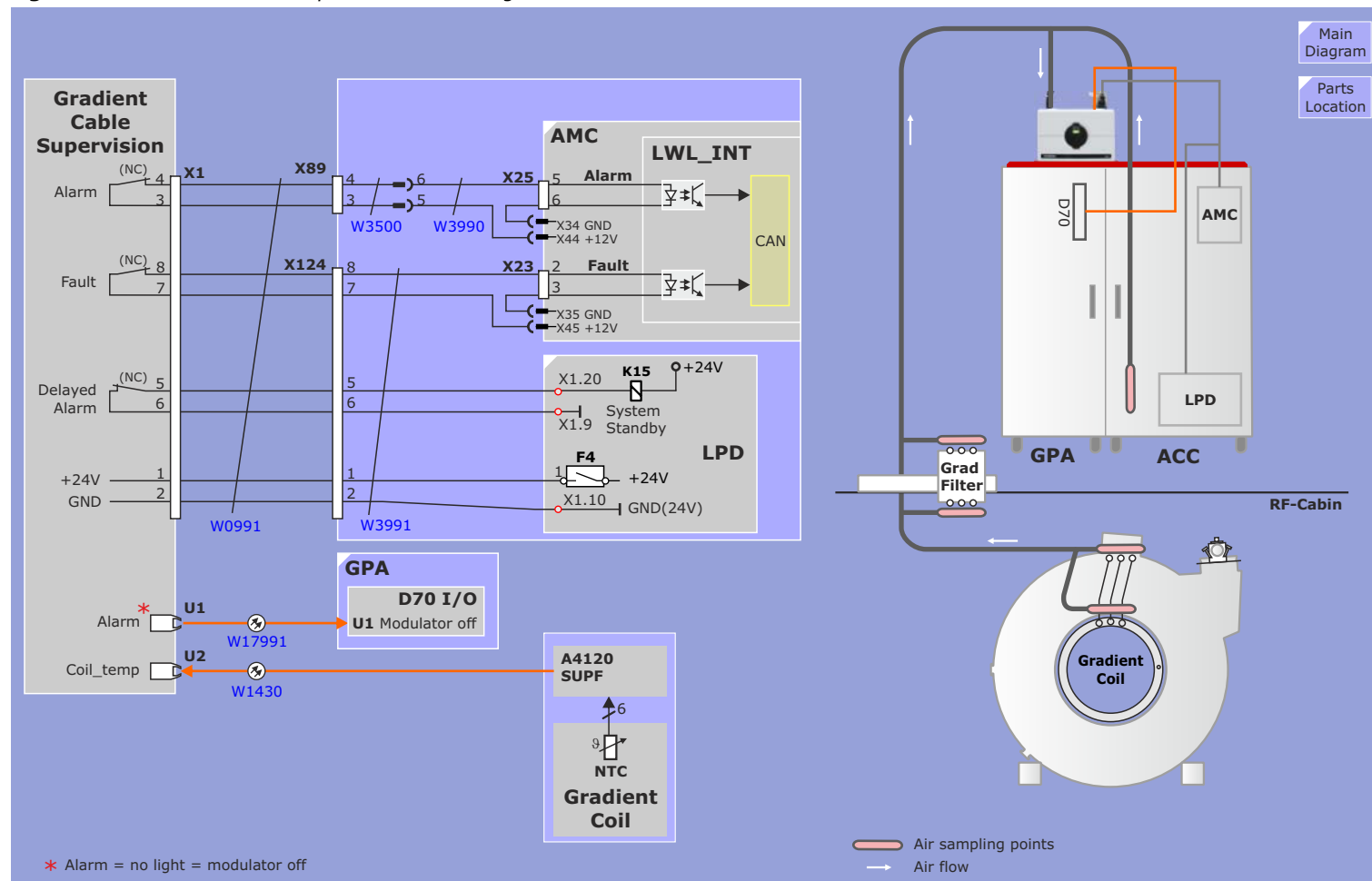
Figure 156 Gradient Cable Supervision Block Diagram
