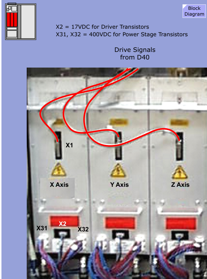
Figure 150 Power Stage Modules
